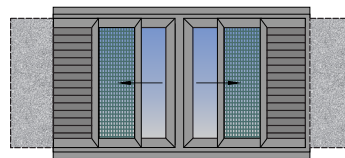
Two sash pocket with fly-screen & shutter
